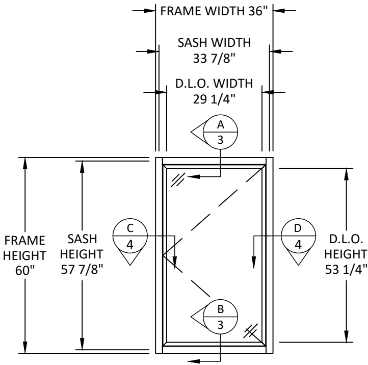
TYPICAL ELEVATION
