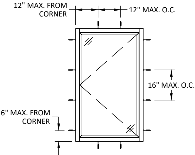
ANCHOR LAYOUT
